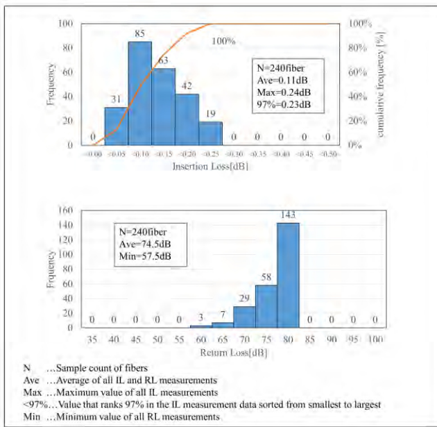
Figure 4. IL and RL of the MMC connectors with 16 single-mode fibers.
